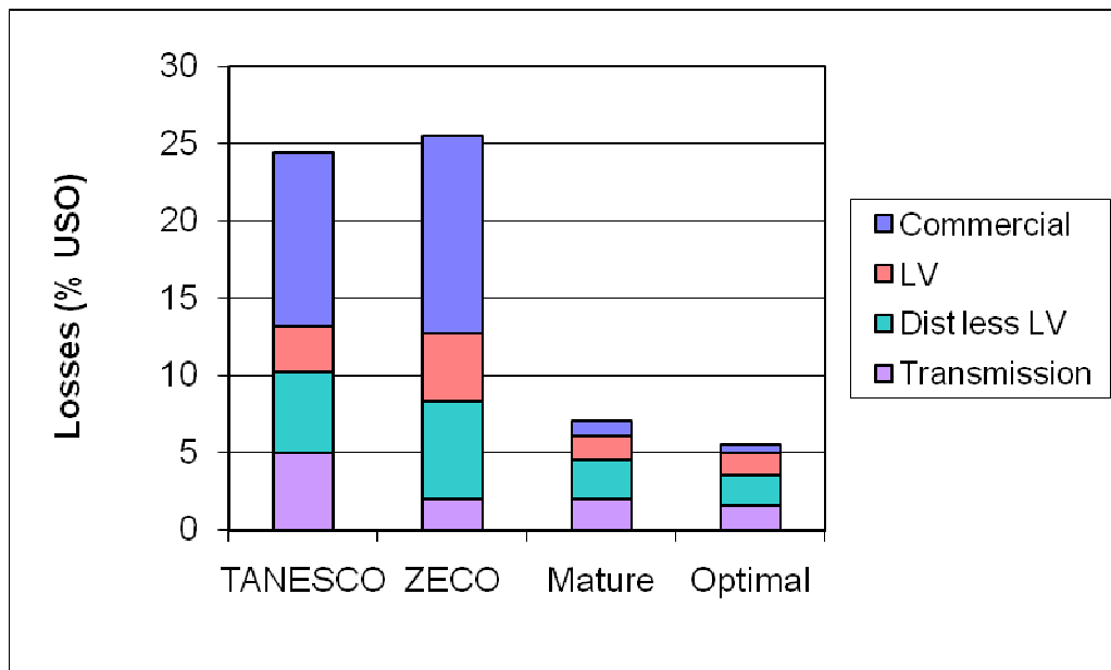
Figure 3.9 – Total T&D Loss Composition
