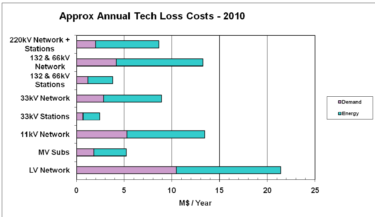
Figure 3.4 – TANESCO T&D Technical Loss Costs – 2010
