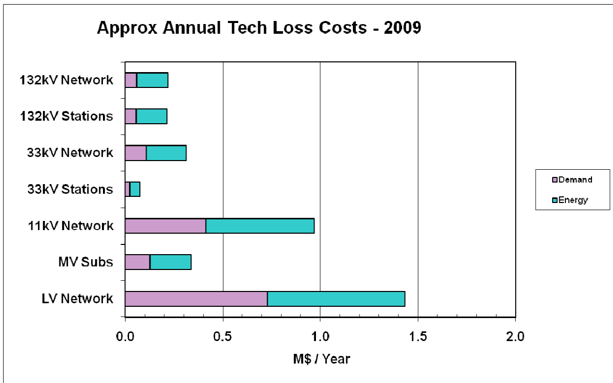
Figure 3.8 – ZECO Technical Loss Costs – 2009
